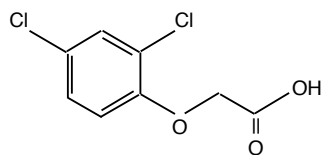
2,4-dichlorophenoxyacetic acid
